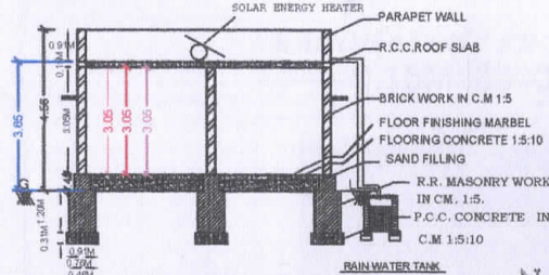
SECTION - XX
