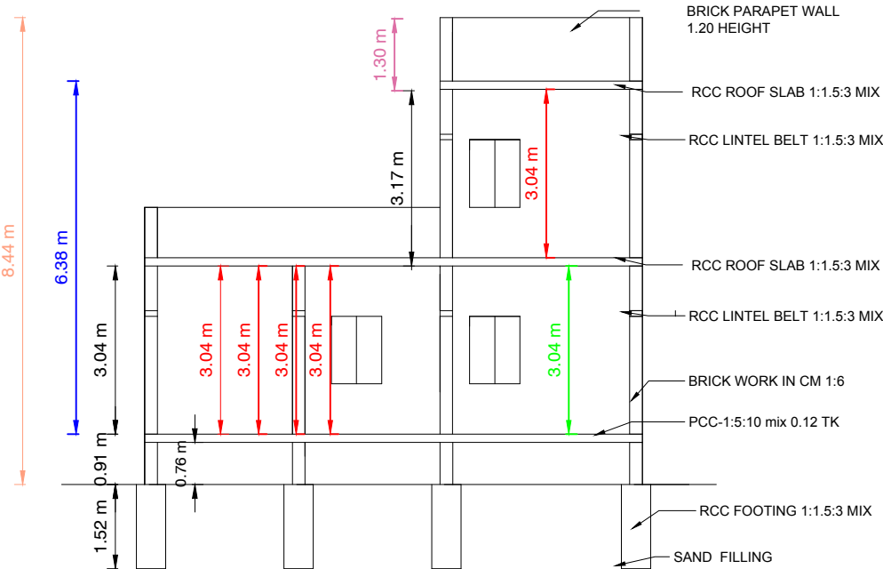
SECTION "AB"
