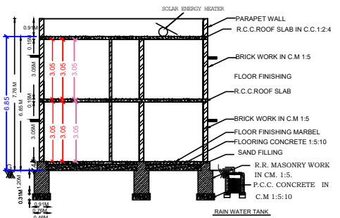
SECTION - XX
