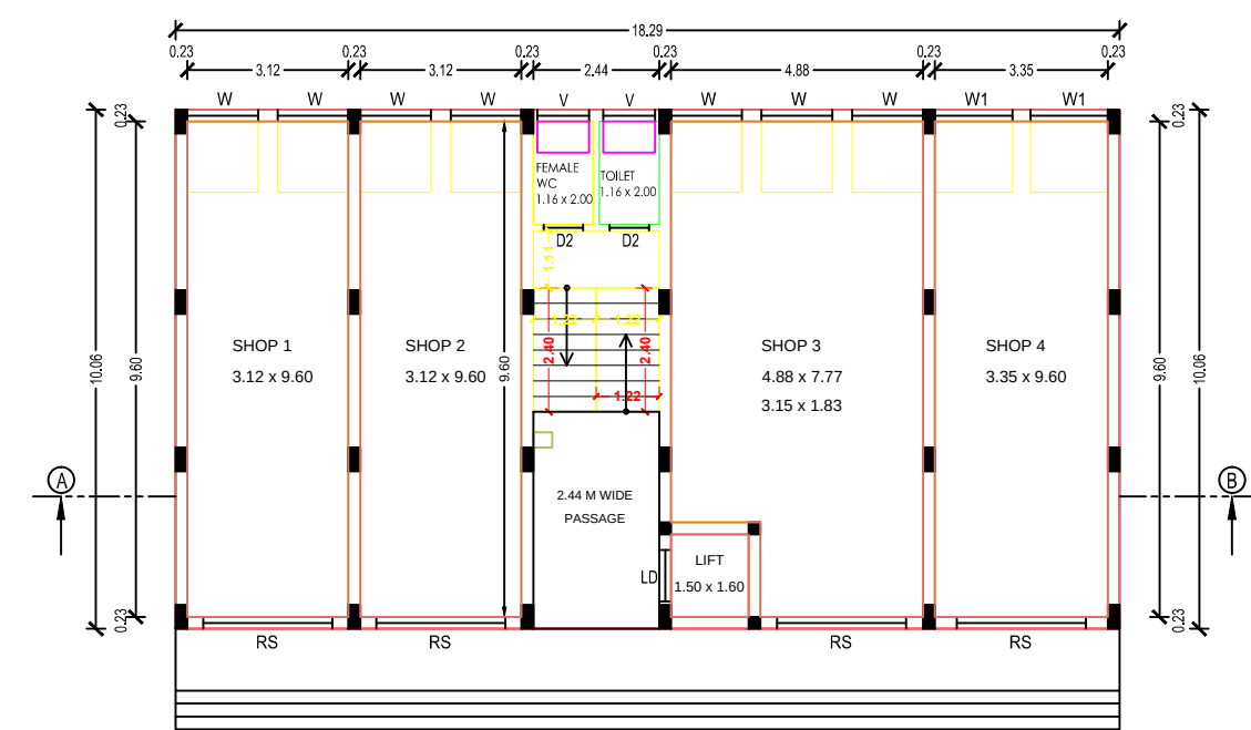
GROUND FLOOR PLAN (PROPOSED COMMERCIAL BUILDING)
