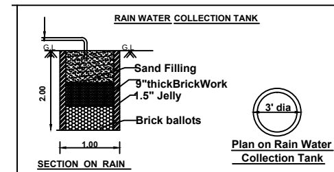
SECTION ON RAIN Plan on Rain Water Collection Tank
