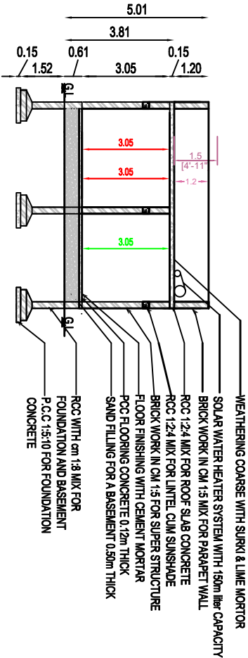
SECTION-"AA"
