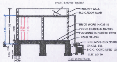
SECTION-XY
