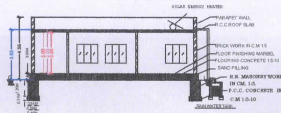
SECTION - XX
