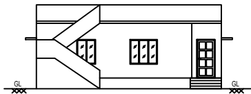
ELEVATION - EAST FACING
