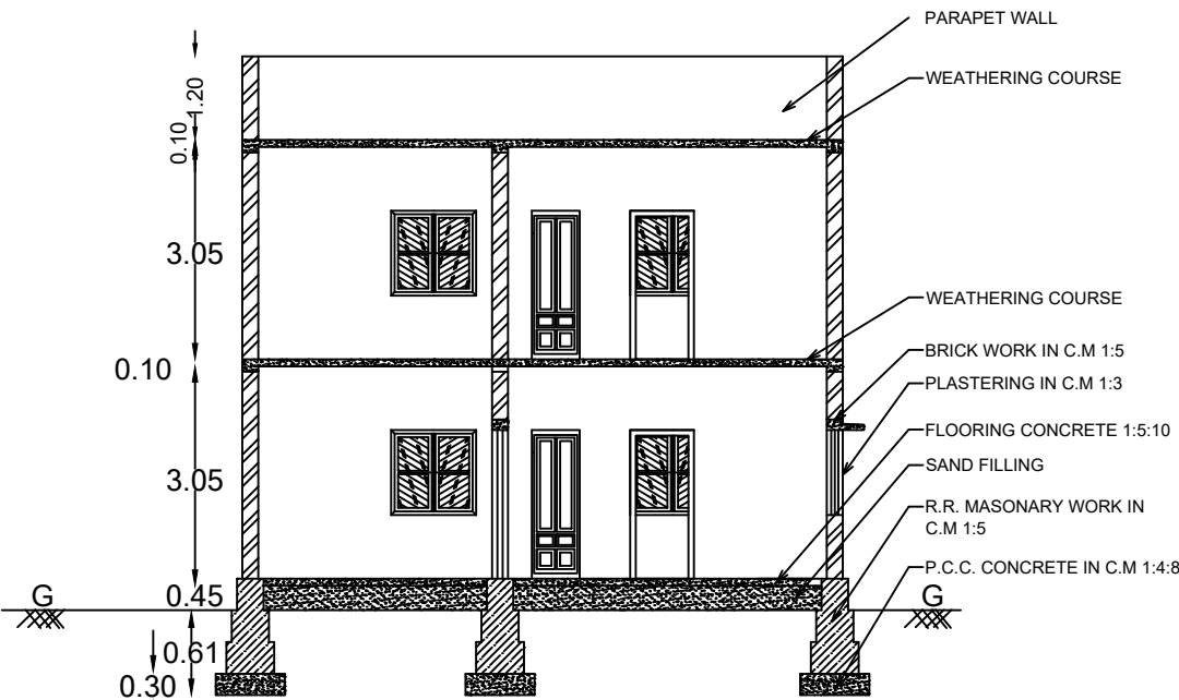
SECTION - XY
