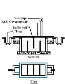
FOUNDATION DETAIL - A
