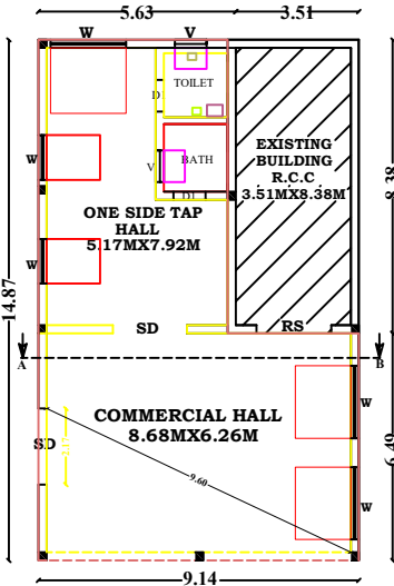
COMMERCIAL BUILDING - PLAN - I
