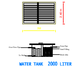
WATER TANK 2000 LITER
