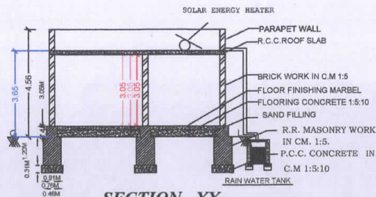
SECTION - XX
