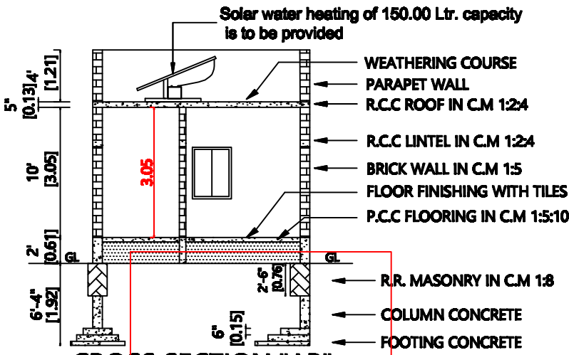
CROSS SECTION "AB"
