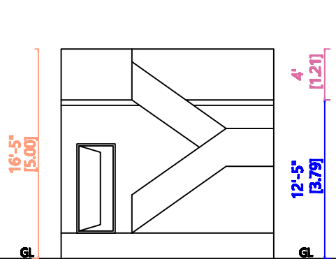
FRONT ELEVATION (NORTH SIDE VIEW)
