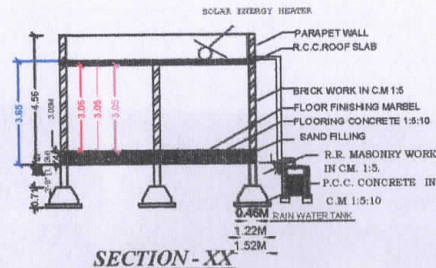
SECTION - XX'
