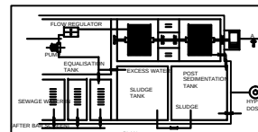
THE TREATMENT PLANT DETAILS
