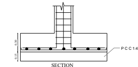
LINTEL BEAM SECTION
