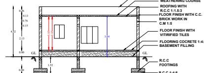
SECTION ON "S-S"
