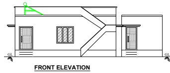
FRONT ELEVATION
