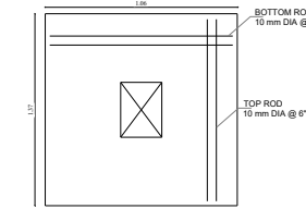
FOOTING PLAN
