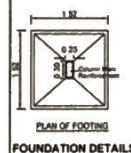
FOUNDATION DETAILS
