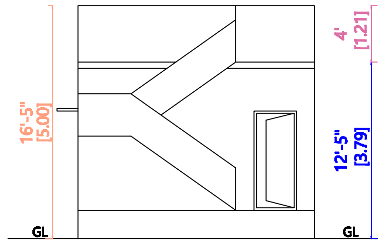
FRONT ELEVATION (EAST SIDE VIEW)
