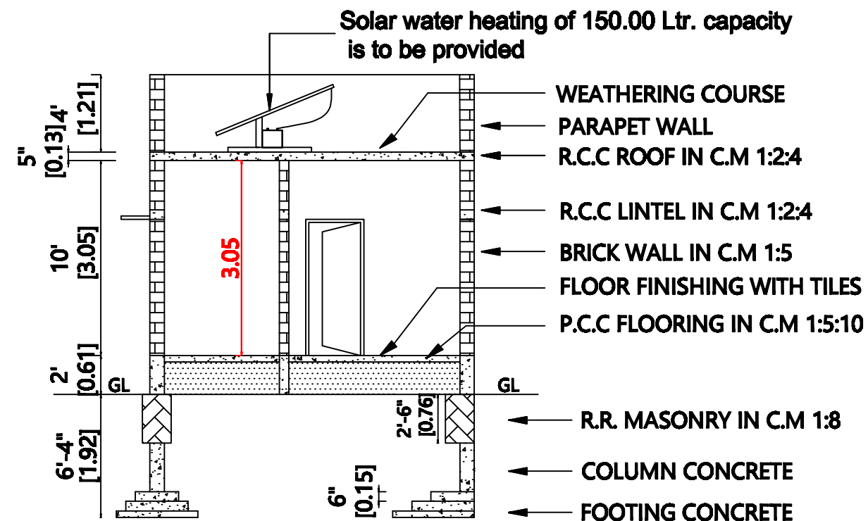
CROSS SECTION "AB"
