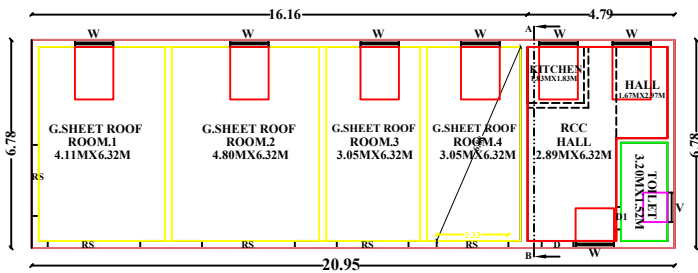
GROUND FLOOR COMMERCIAL CUM RESIDENTIAL - PLAN
