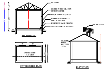
CATTLE SHED-PLAN
