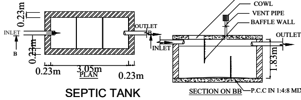
SEPTIC TANK
