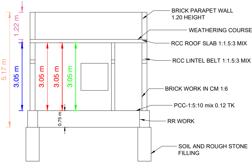
SECTION"AB"
