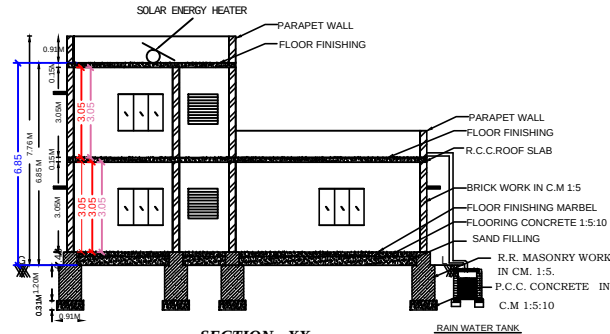
SECTION - XX
