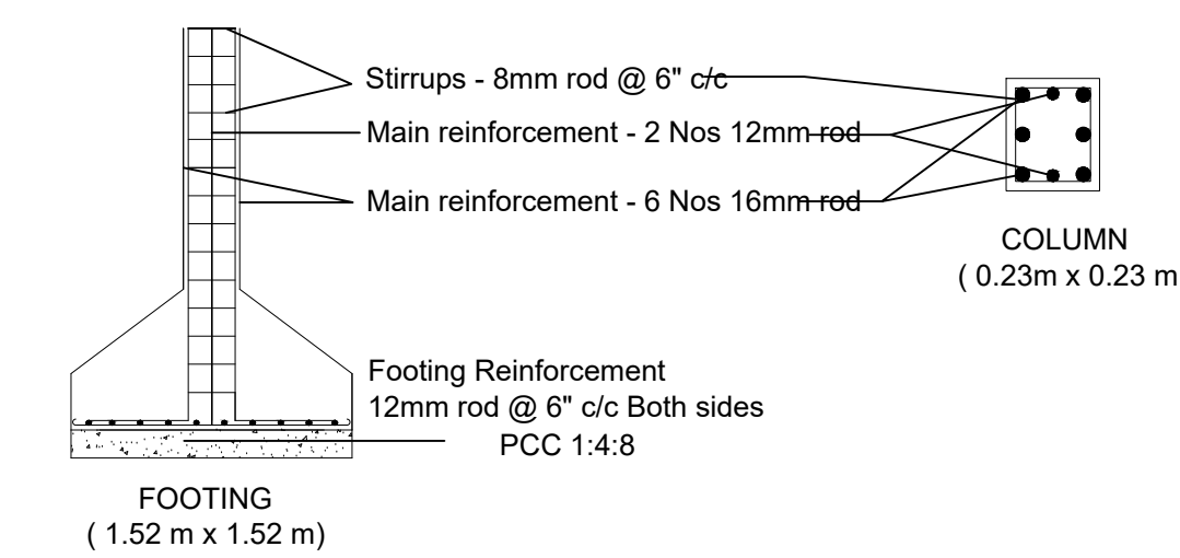
Column &amp; Footing Reinforcement Details
