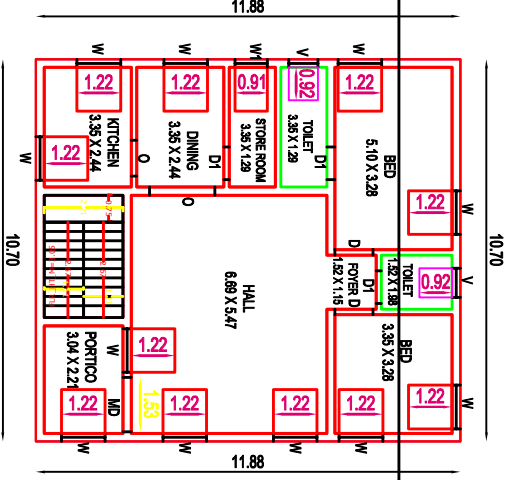
FIRST FLOOR PLAN (Scale 1:100)
