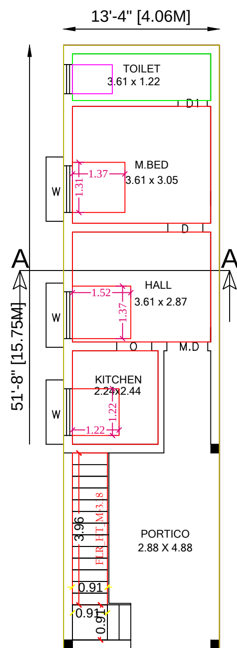
PLAN- GROUND FLOOR
