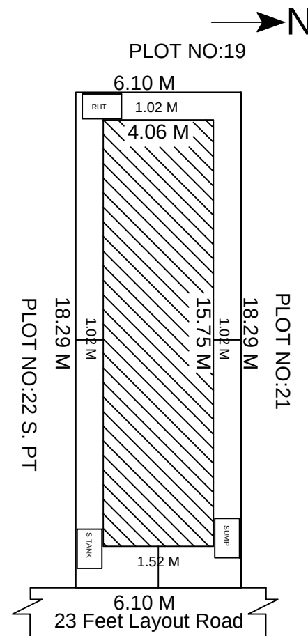
PLAN- FIRST FLOOR
