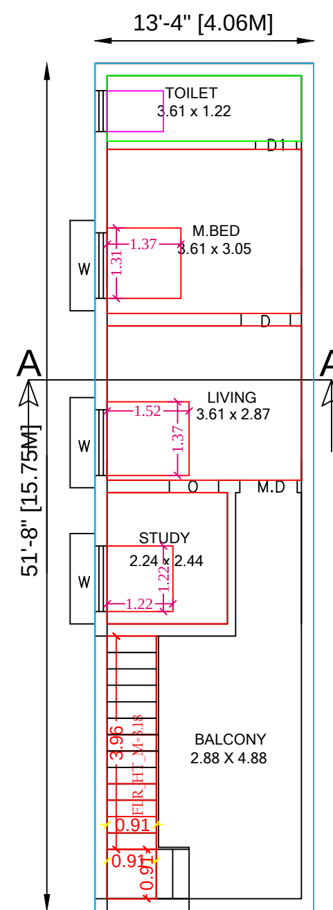
PLAN- FIRST FLOOR
