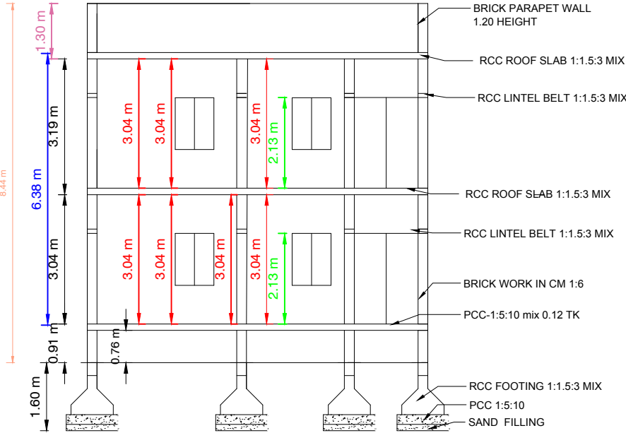
SECTION "AB"
