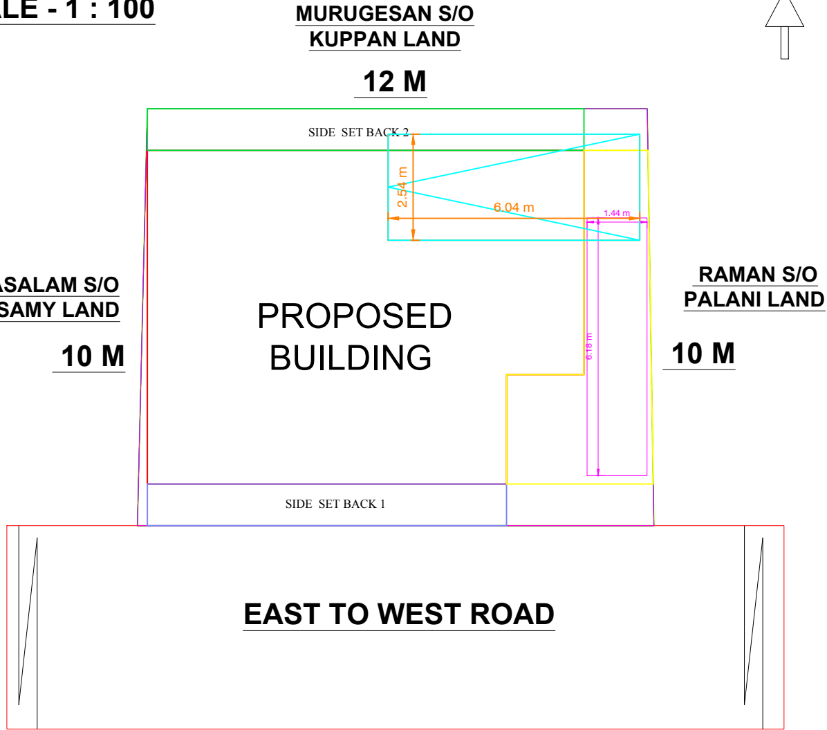
TOPO PLAN
