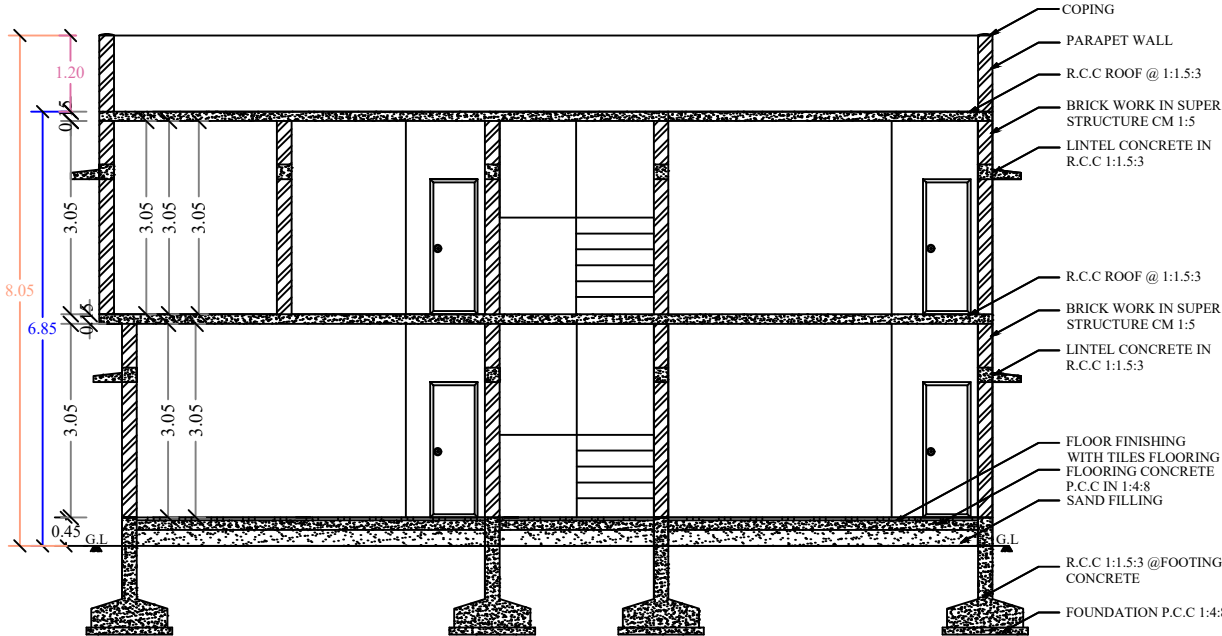
SECTION-AB
