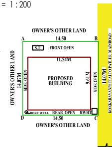
SITE PLAN
