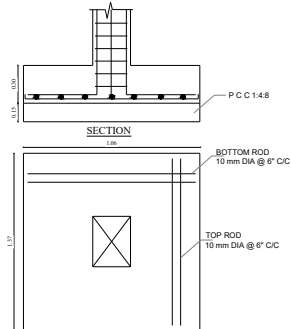
FOOTING PLAN
