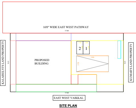
SITE PLAN
