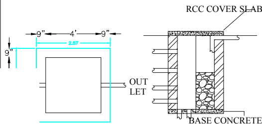
PLAN SECTION RAIN WATER COLLECTION PIT DETAILS NOT TO SCALE
