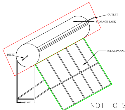
NOT TO SCALE SOLAR WATER HEATER DETAILS
