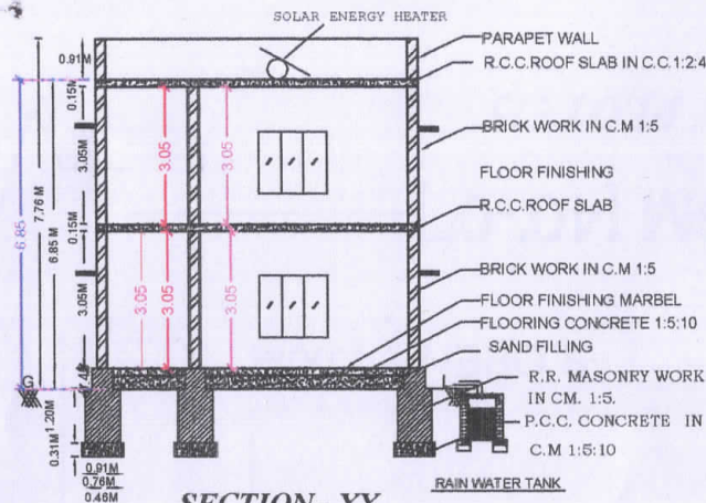
SECTION - XX
