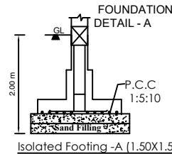
Isolated Footing - A (1.50X1.50) (Not to Scale)
