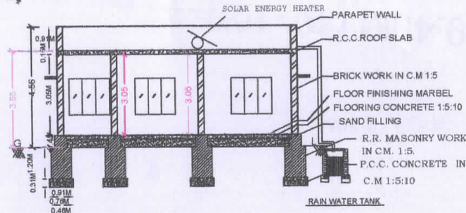
SECTION - XX
