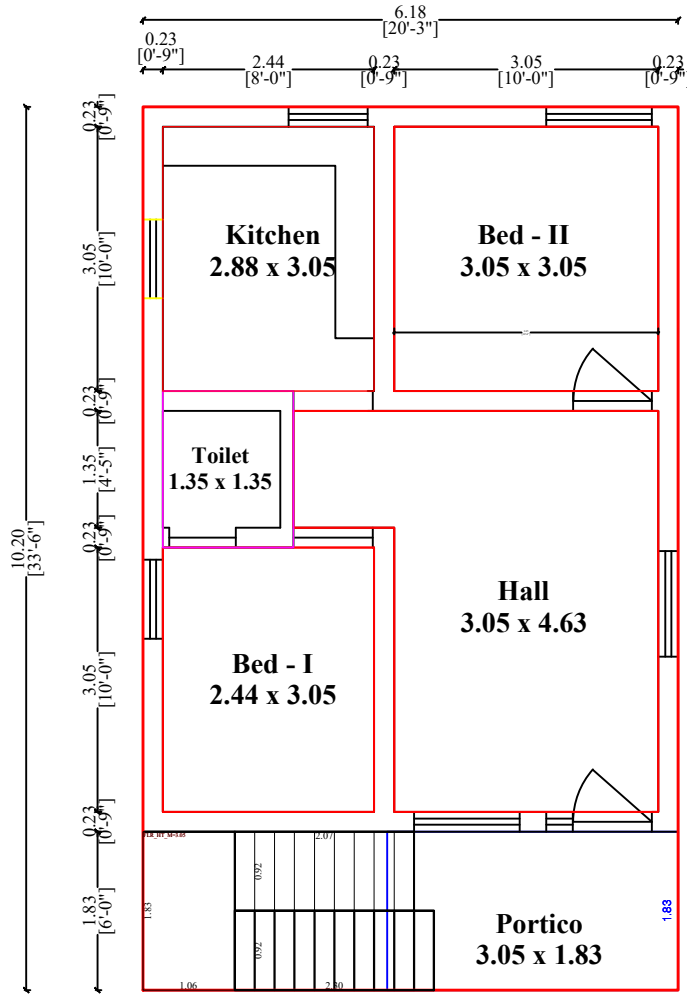
Building Plan (Scale 1:100)
