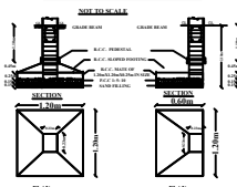
TYP.DET. COLUMN FOOTING
