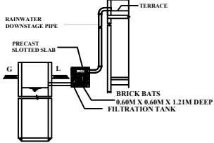
RAIN WATER HARVESTING SYSTEM
