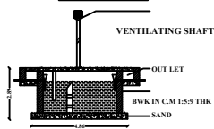
SECTION OF THE SEPTIC TANK
