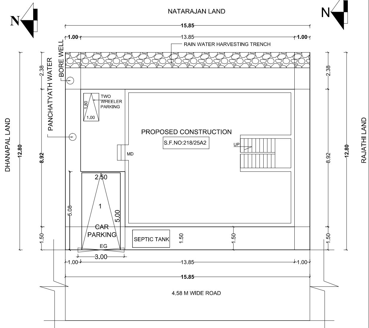
SITE PLAN
