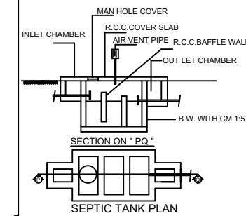
SEPTIC TANK PLAN
