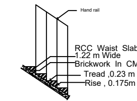
STAIRCASE DETAILS SECTION
