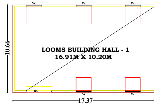
COMMERCIAL PLAN-I [LOOMS BUILDING]
