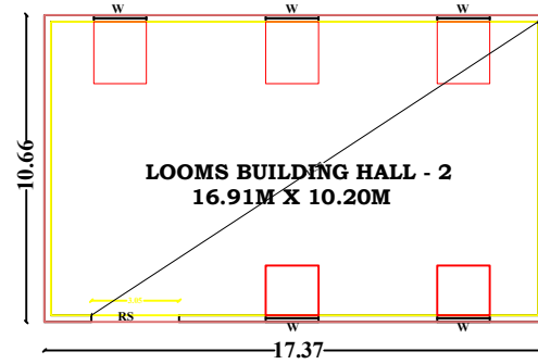
COMMERCIAL PLAN-II [LOOMS BUILDING]
