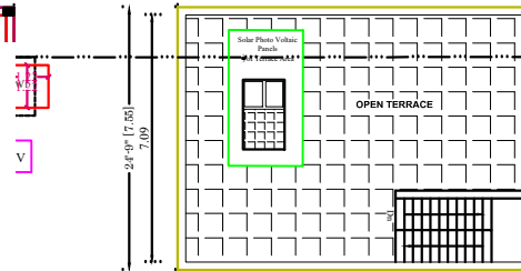
ROOF FLOOR PLAN SCALE:1:100
