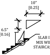
STAIR CASE DETAILS
