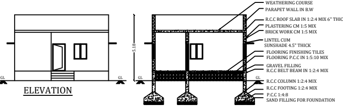
SECTION AB
