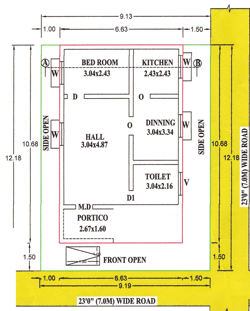
GROUND PLAN
