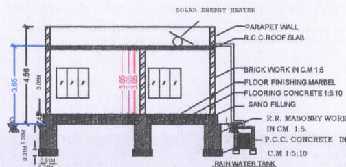
SECTION - XX
