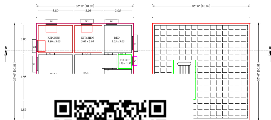
OOF FLOOR PLAN SCALE - 1:100
