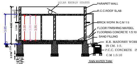
SECTION - XX
