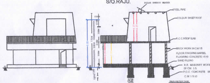
SECTION-XX
