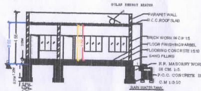
SECTION - XX
