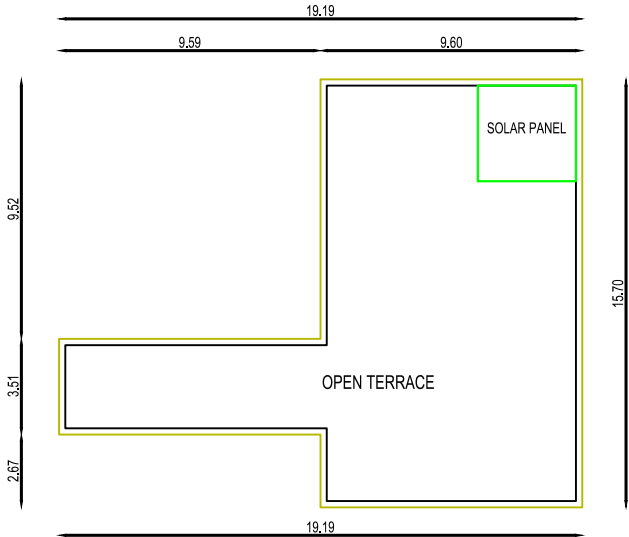
PROPOSED TERRACE FLOOR PLAN (Scale 1:100)
