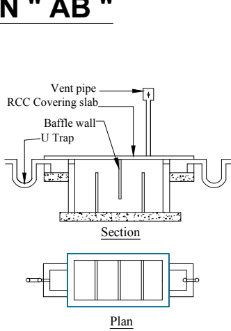
SECTION " AB "
