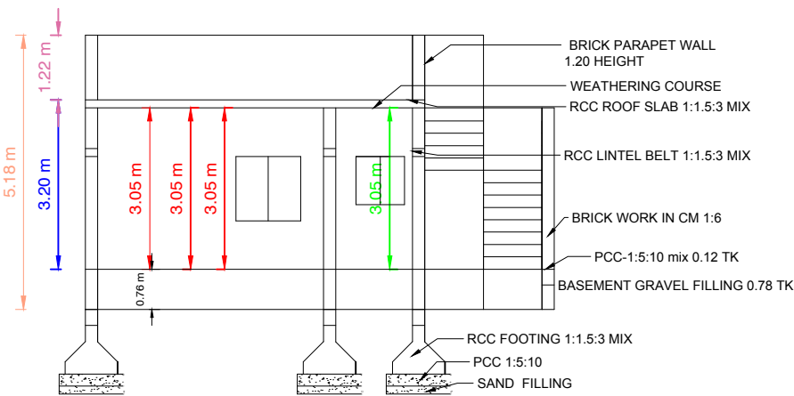
SECTION " AB "
