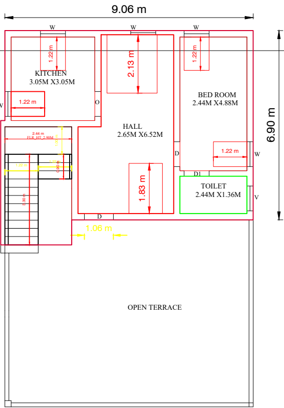
PRO-SECOND FLOOR PLAN
